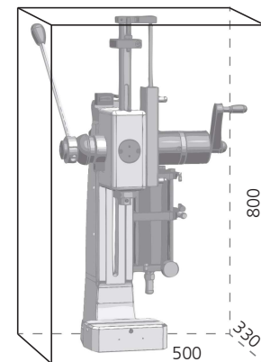
Volume dimensions with frame no. 5
