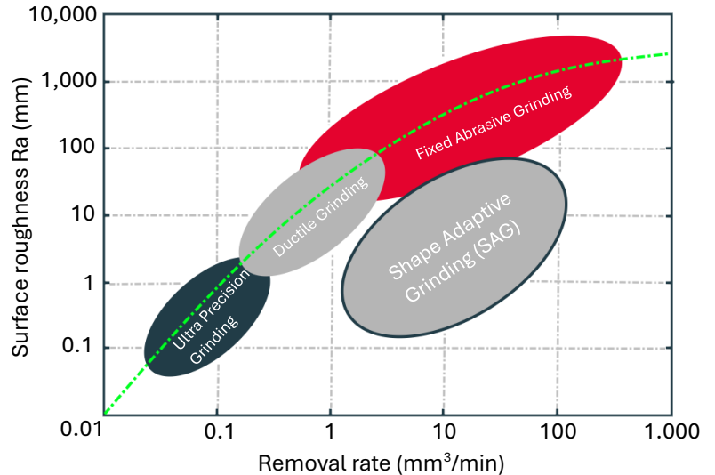
Comparison of conventional and shape adaptive grinding
