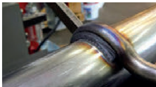
HD-MAG welding process
