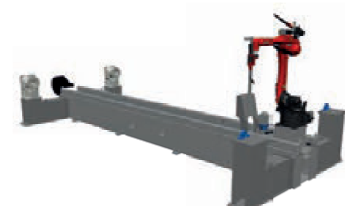
TRACK-FRAME-H
