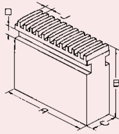
SOFT
