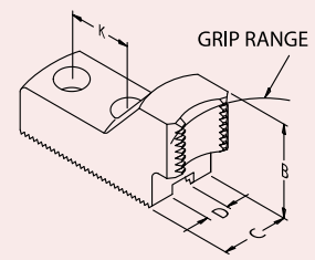
BAR GRIPPING
