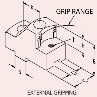
EXTERNAL GRIPPING
